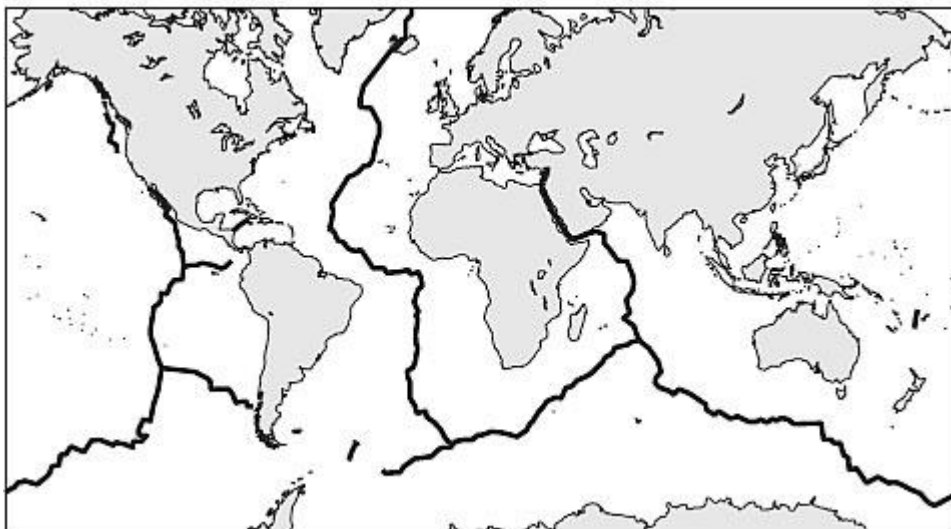
Mid-Ocean Ridges
